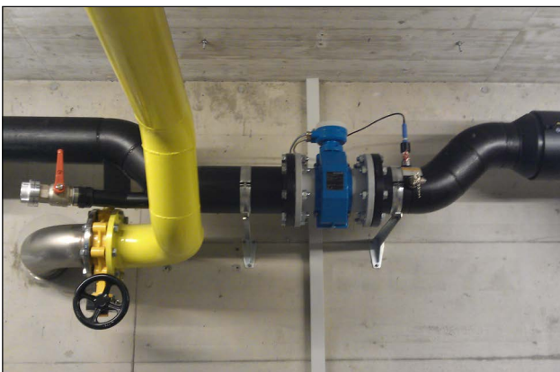
Stationary flow meter 150 nominal diameter installed in the sewer discharge line
